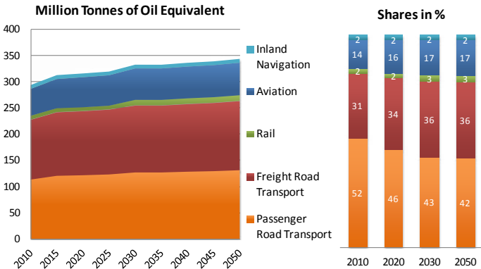
Final energy demand in transport 2010 - 2050
