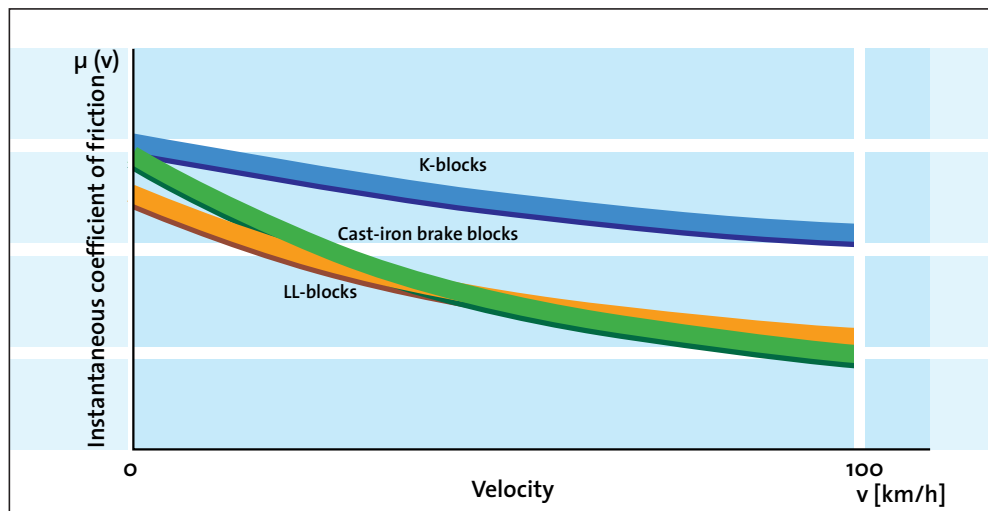
Figure 3.2.2: Coefficient of friction for different brake blocks at different speeds. The graph shows the higher coefficient of friction of K-blocks and the similar performance of LL and cast iron brake blocks.
