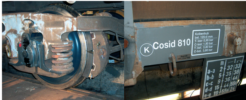
Figure 3.2.1: Picture of wagon retrofitted with k-blocks. Old wagons such as these are now as silent as modern passenger vehicles.
